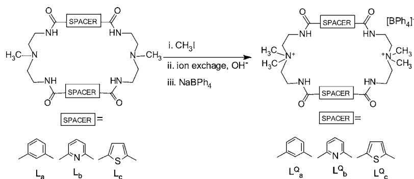
Scheme 1. Synthetic Pathway of Mixed Amide/Quaternary Amine Macrocycles, L_{a-c}^{Q_{a-c} 2+}
